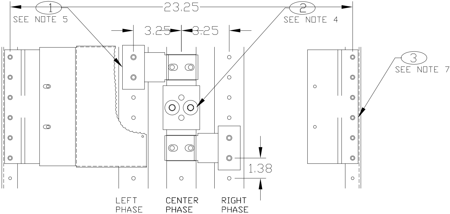
FRONT VIEW SHOWING MOUNTING LOCATIONS OF CONNECTIONS TO BUS BARS AND BREAKER MOUNTING BRACKET TO "Z" RAILS (BREAKER REMOVED TO SHOW CONNECTORS)
