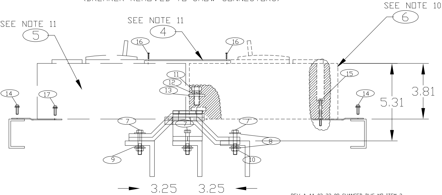
FRONT VIEW SHOWING MOUNTING LOCATIONS OF CONNECTIONS TO BUS BARS AND BREAKER MOUNTING BRACKET TO "Z" RAILS (BREAKER REMOVED TO SHOW CONNECTORS)
